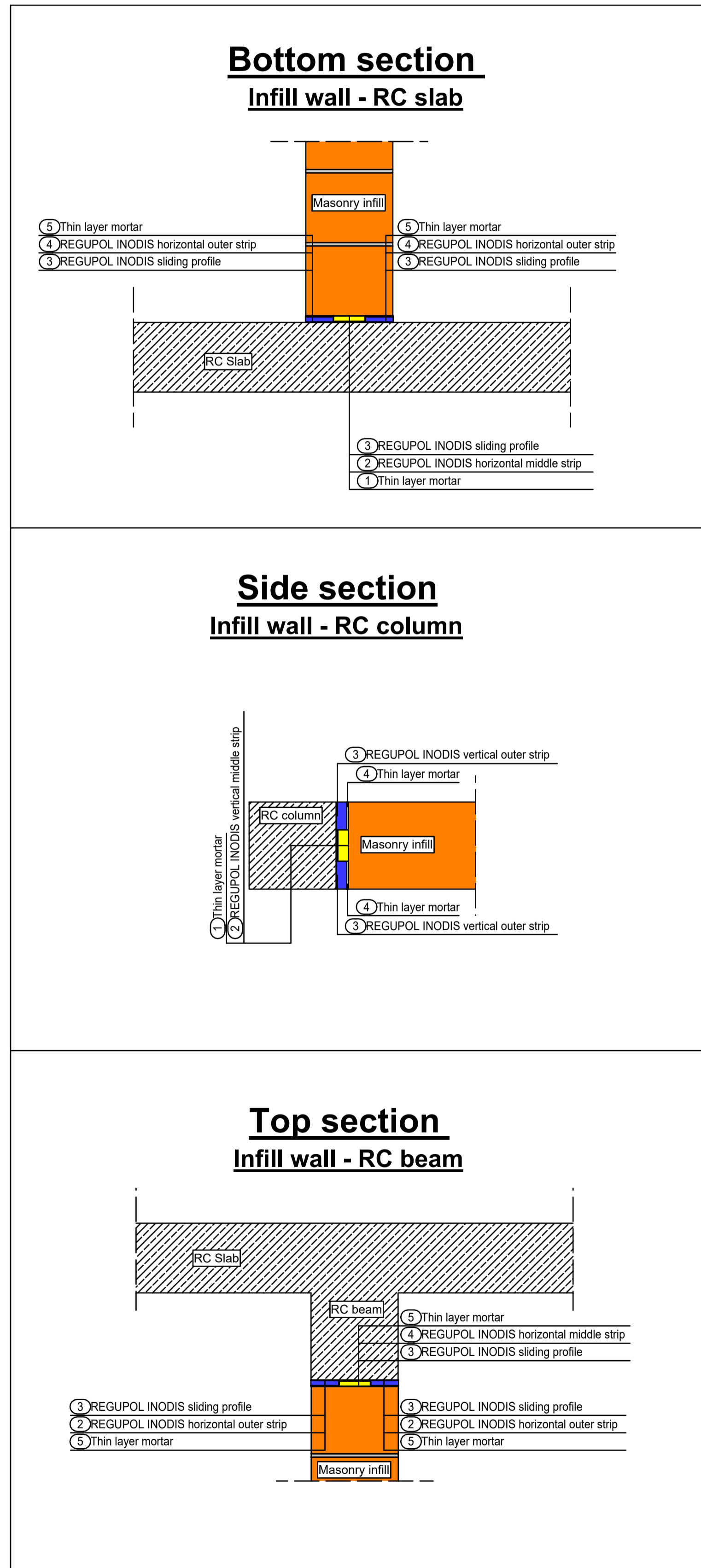
Thickness of the infill wall = Thickness of the RC elements
